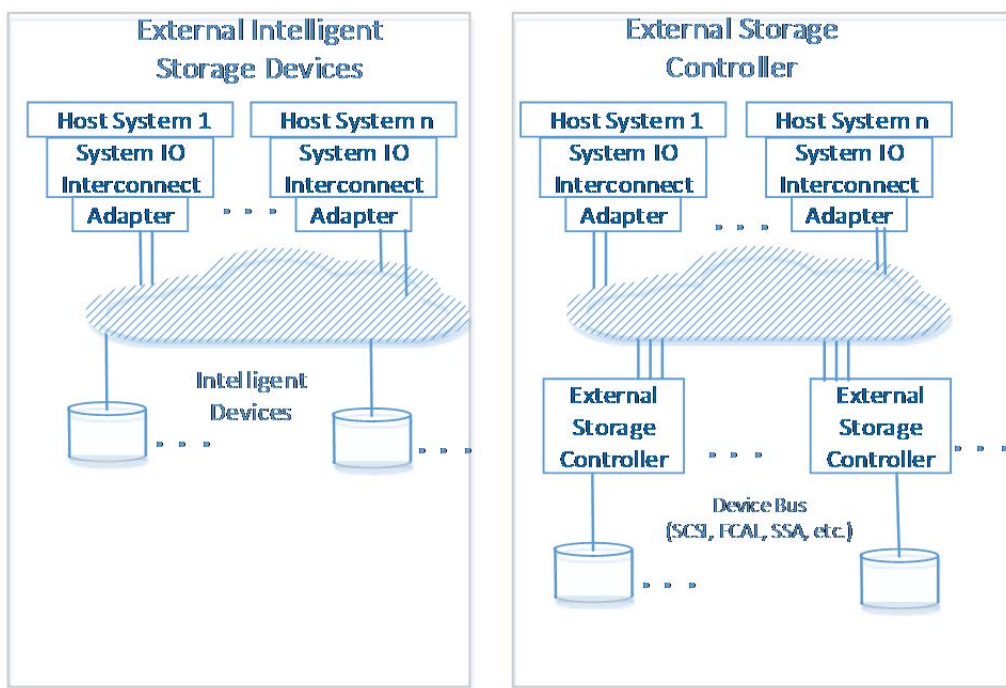
Figure 4-2 External Storage Configurations
