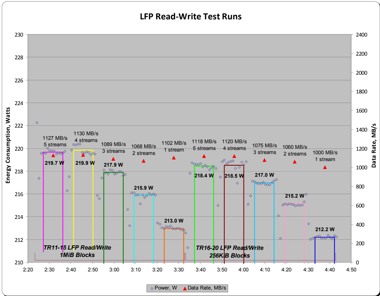
Figure 12-3: SPC-2C/E Large File Processing, READ-WRITE Test Phase
