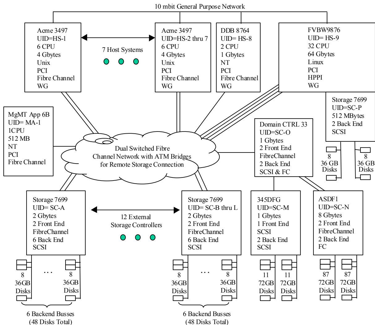
Figure 10-10: Benchmark Configuration/Tested Storage Configuration Diagram
