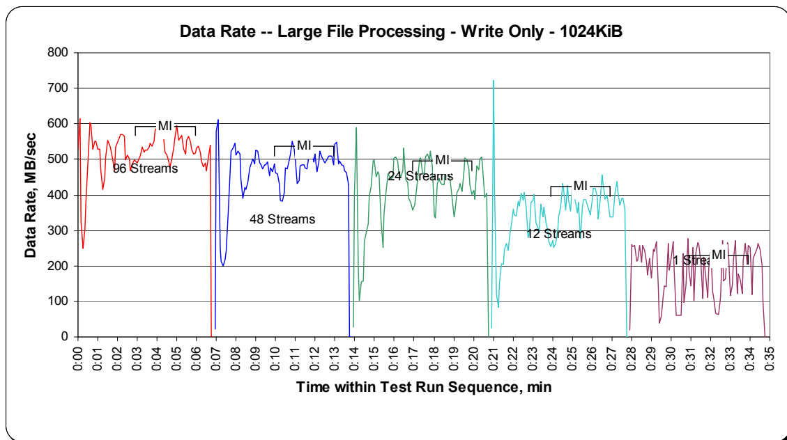
Figure 10-4: Average Data Rate by Interval Graph ( LFP )
