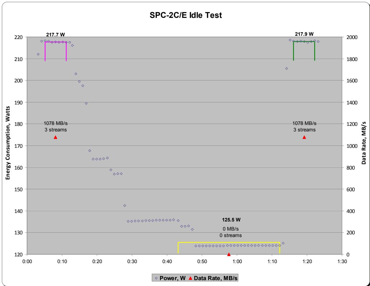
Figure 12-1: SPC-2C/E Idle Test
