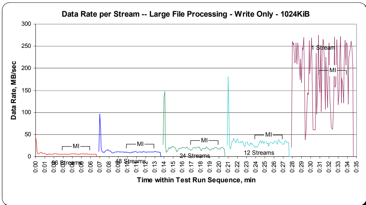
Figure 10-5: Average Data Rate per Stream by Interval Graph ( LFP )
