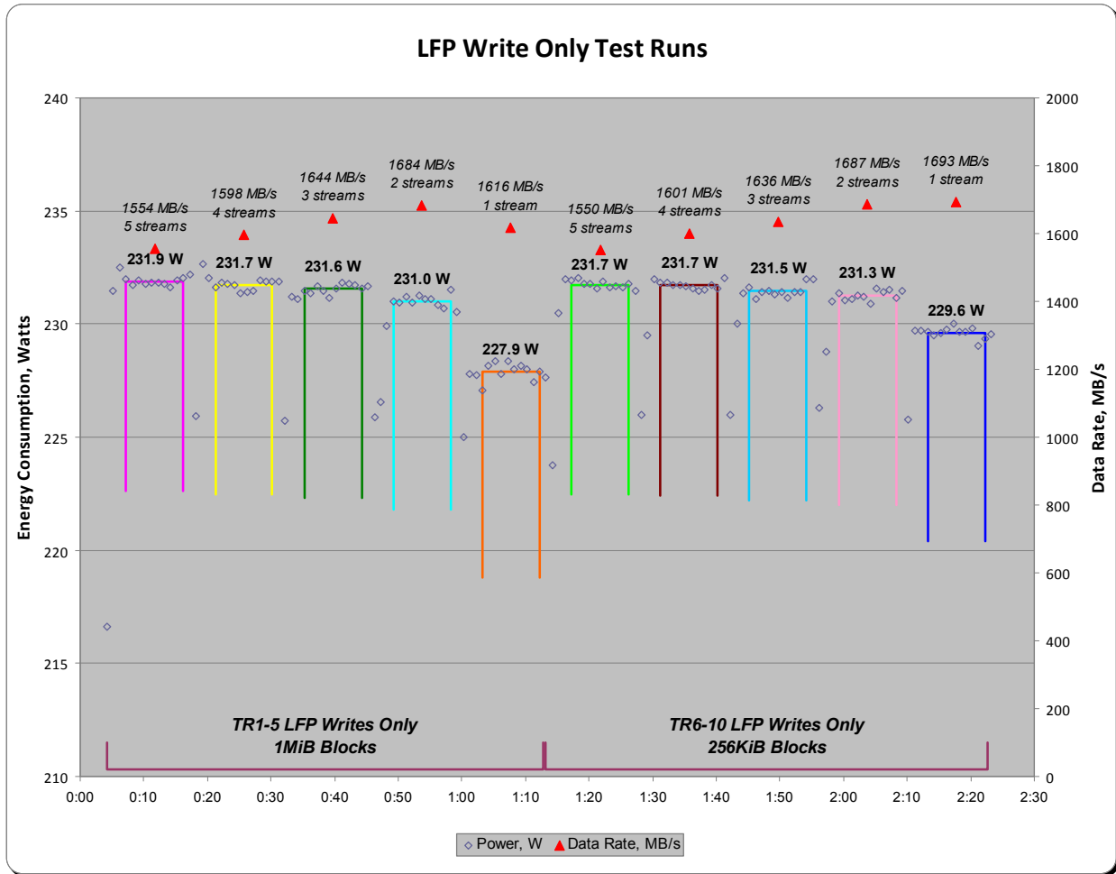
Figure 12-2: SPC-2C/E Large File Processing, WRITE ONLY Test Phase
