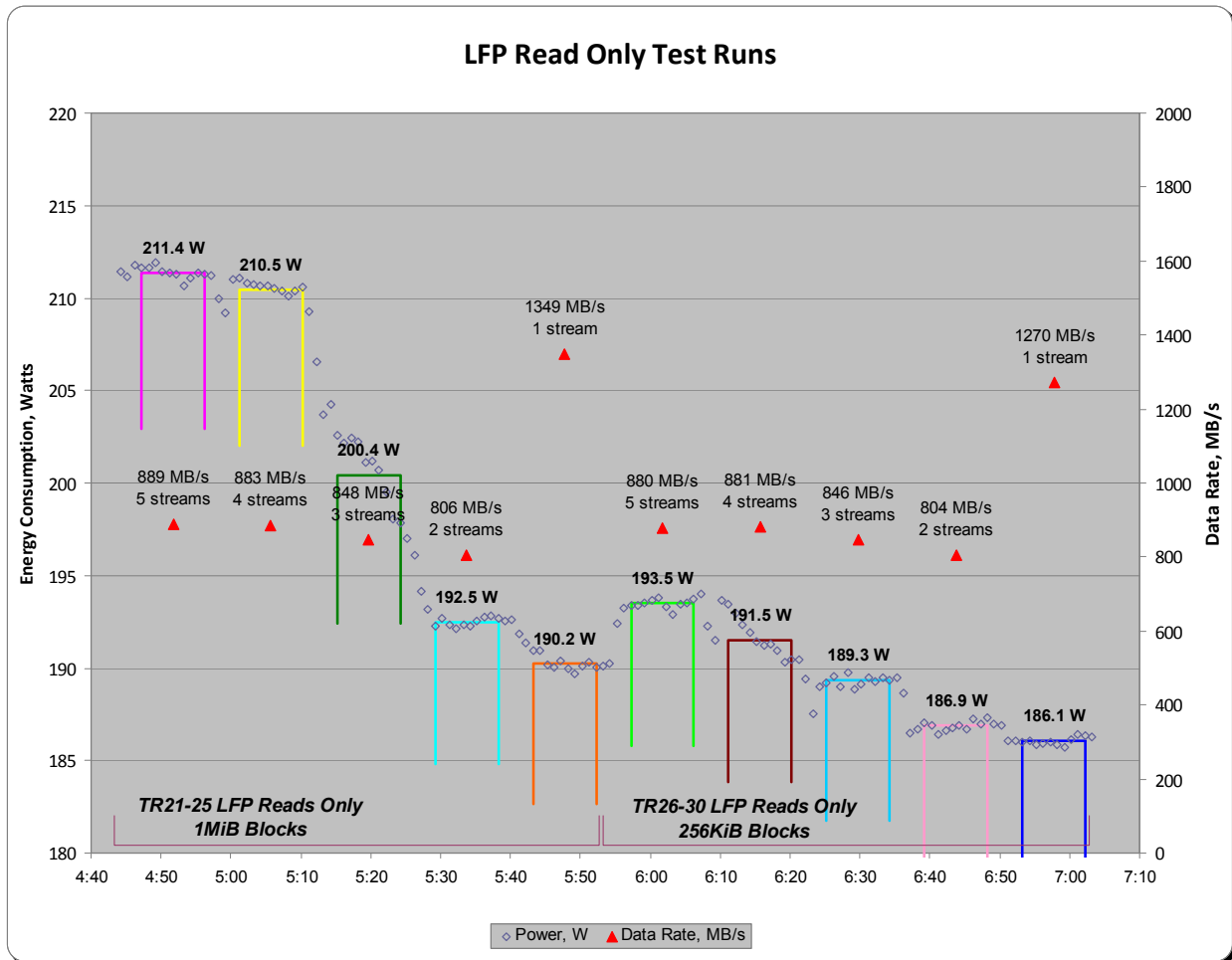
Figure 12-4: SPC-2C/E Large File Processing, READ ONLY Test Phase
