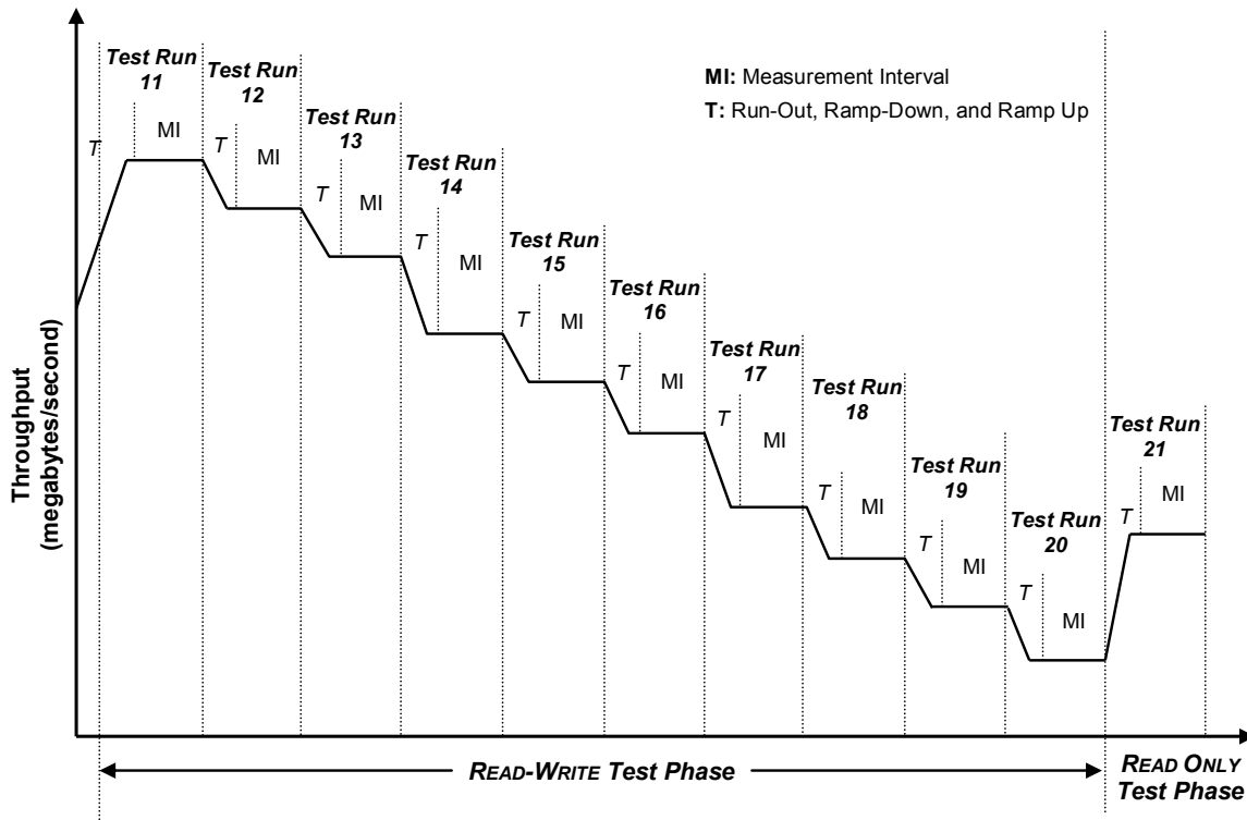
Figure 6-6: Large File Processing READ-WRITE Test Phase
